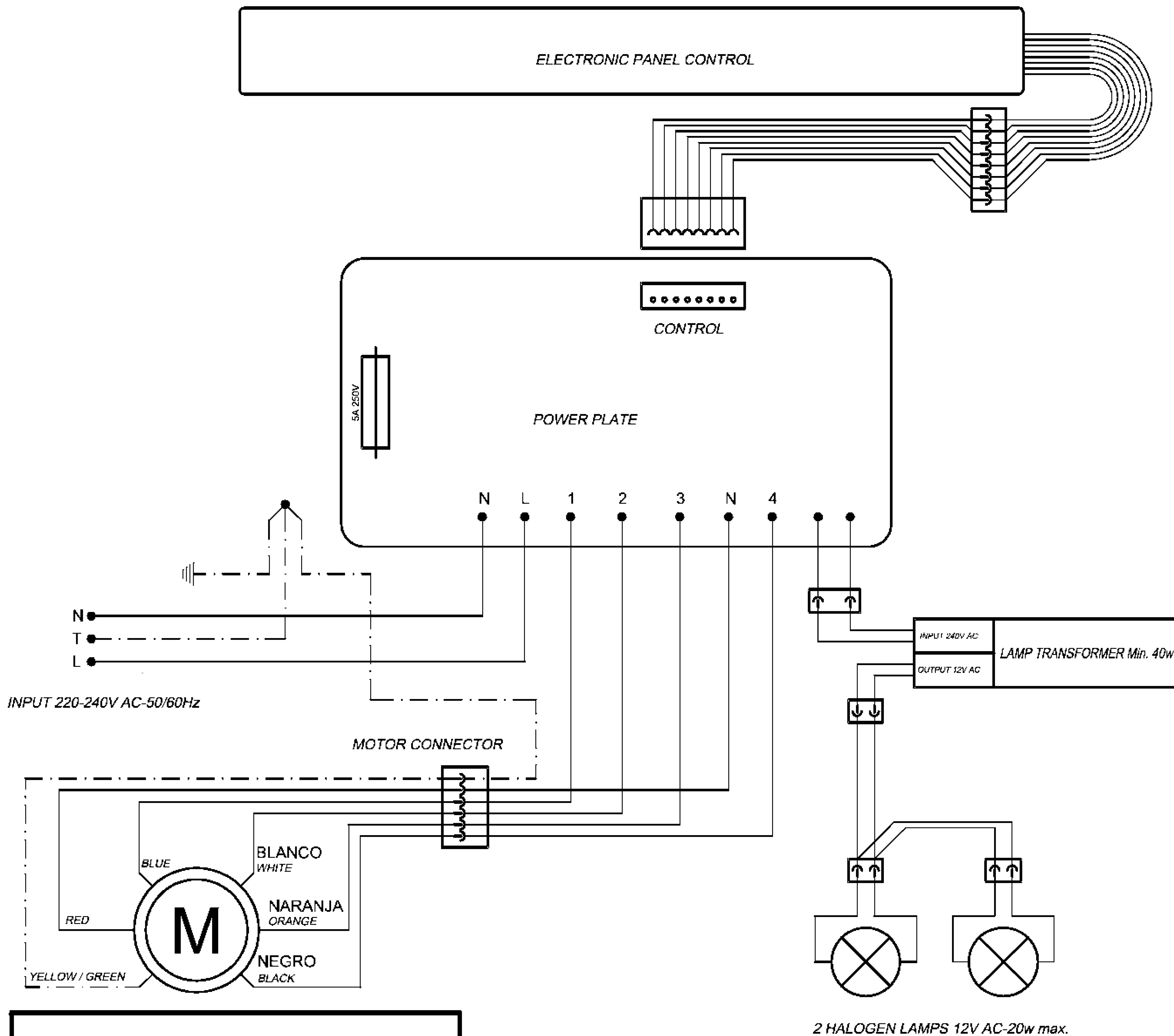
MOTOR CONNECTOR DIAGRAM
